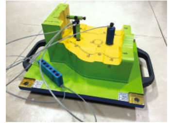
Checking Gauges
